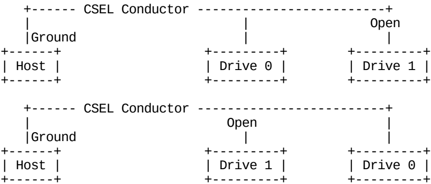
Figure 5 - Cable select
